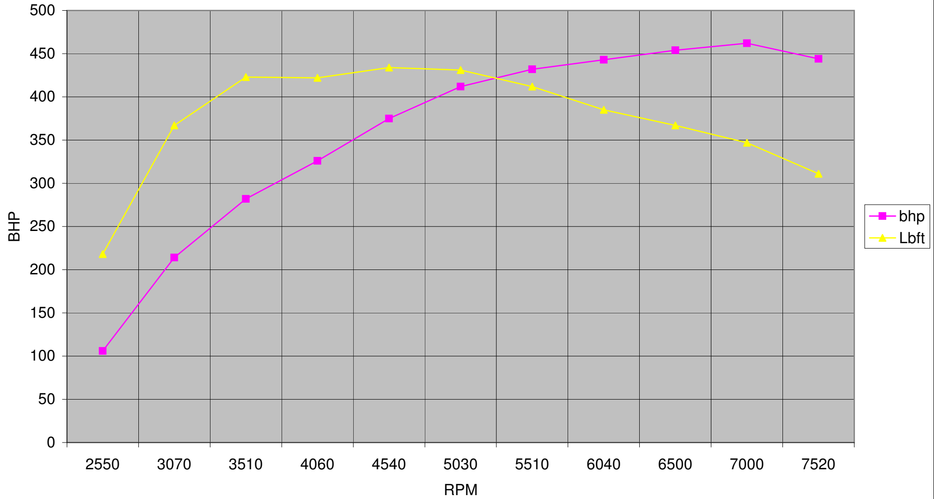
Dyno results of New Engine
